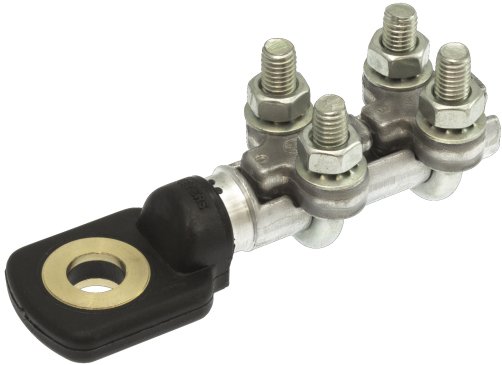
CBM 95
